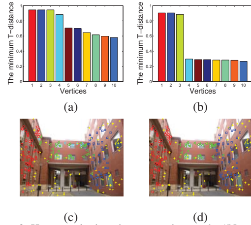
Figure 3. Homography based segmentation on the “Neem” [21]. (a) and (b) The top 10 largest MTD values of the corresponding vertices obtained by the proposed mode seeking algorithm based on G and G^* , respectively. (c) and (d) The segmentation results obtained by the proposed MSH method based on G and G^* , respectively.
